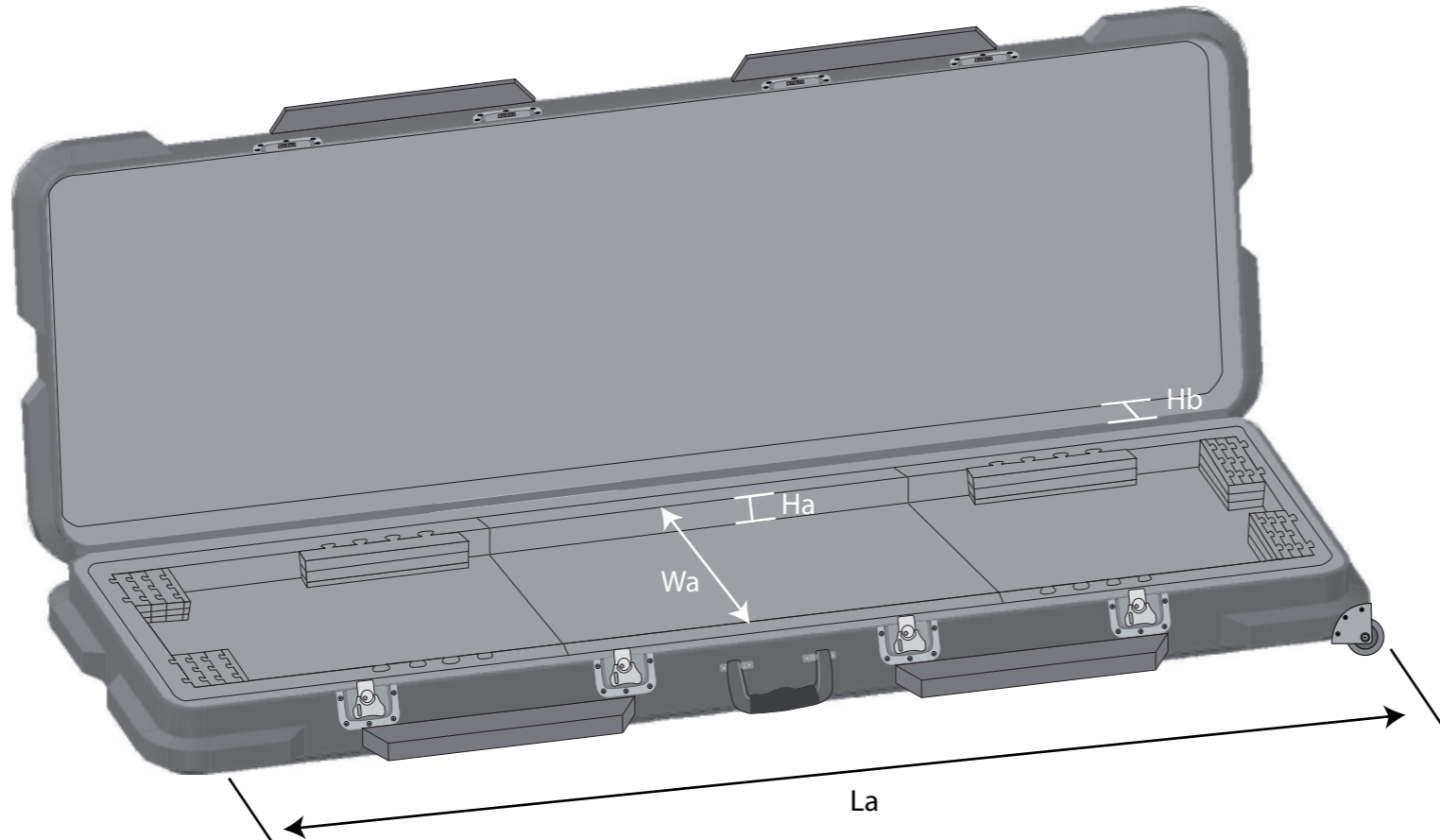
outside ( mm )
